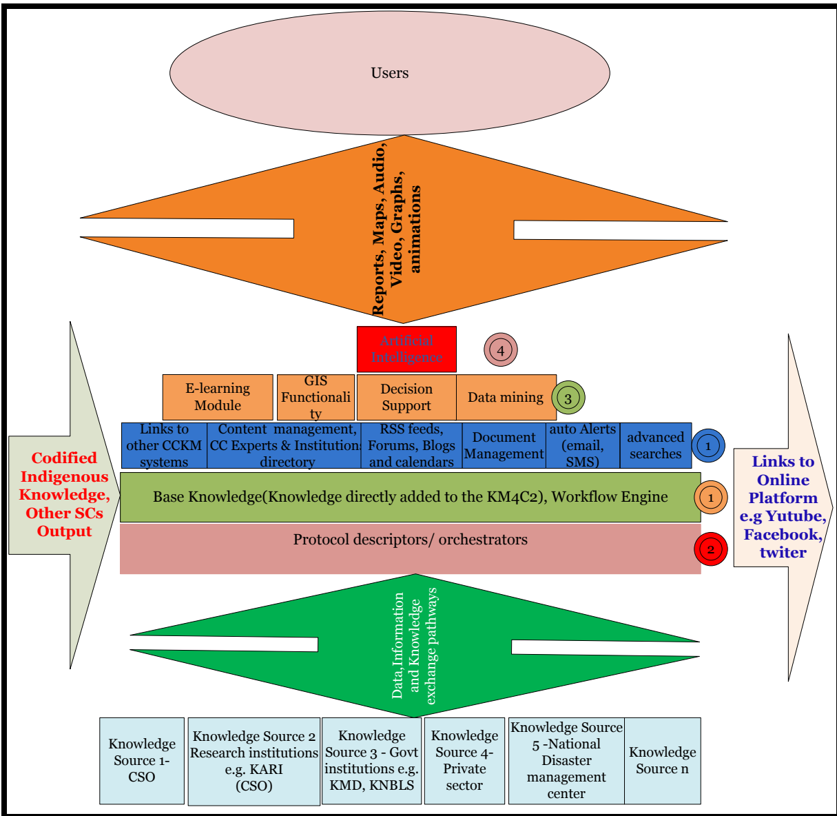
Figure 6: Climate Change Knowledge Management System Conceptual design model
